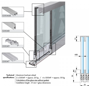
Sliding door cover for glass 6-8 mm
